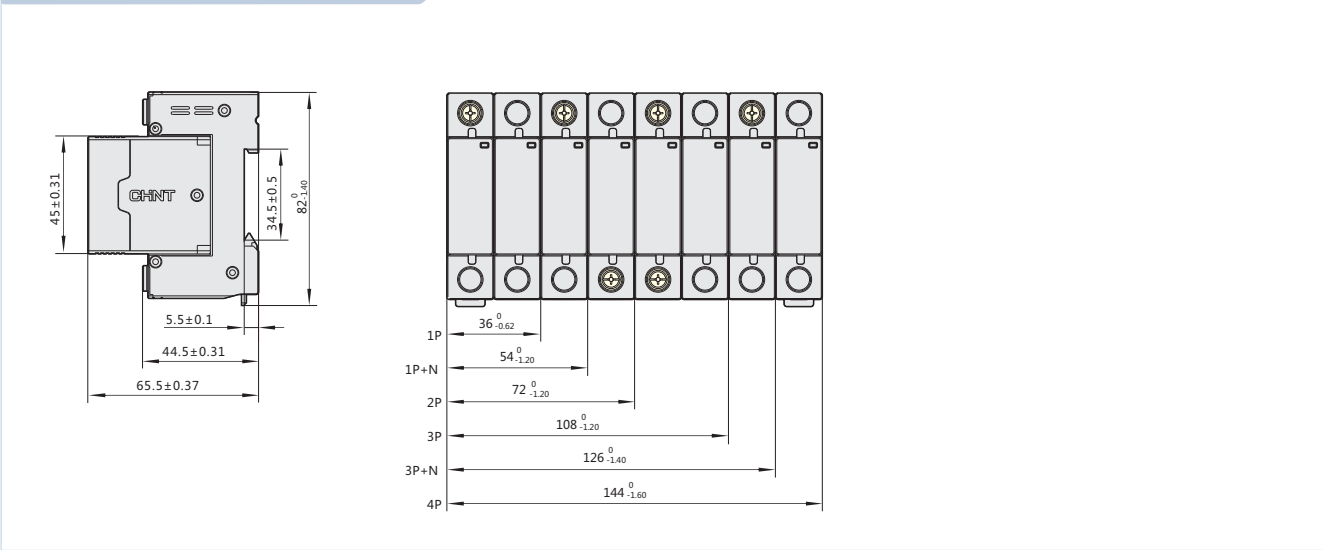
Fig 5 Dimensions and installation sizes of surge protector without remote signal outputs
