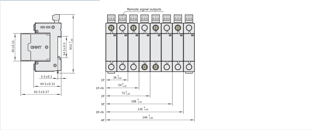
Fig 4 Dimensions and installations sizes of surge protector with remote signal outputs
